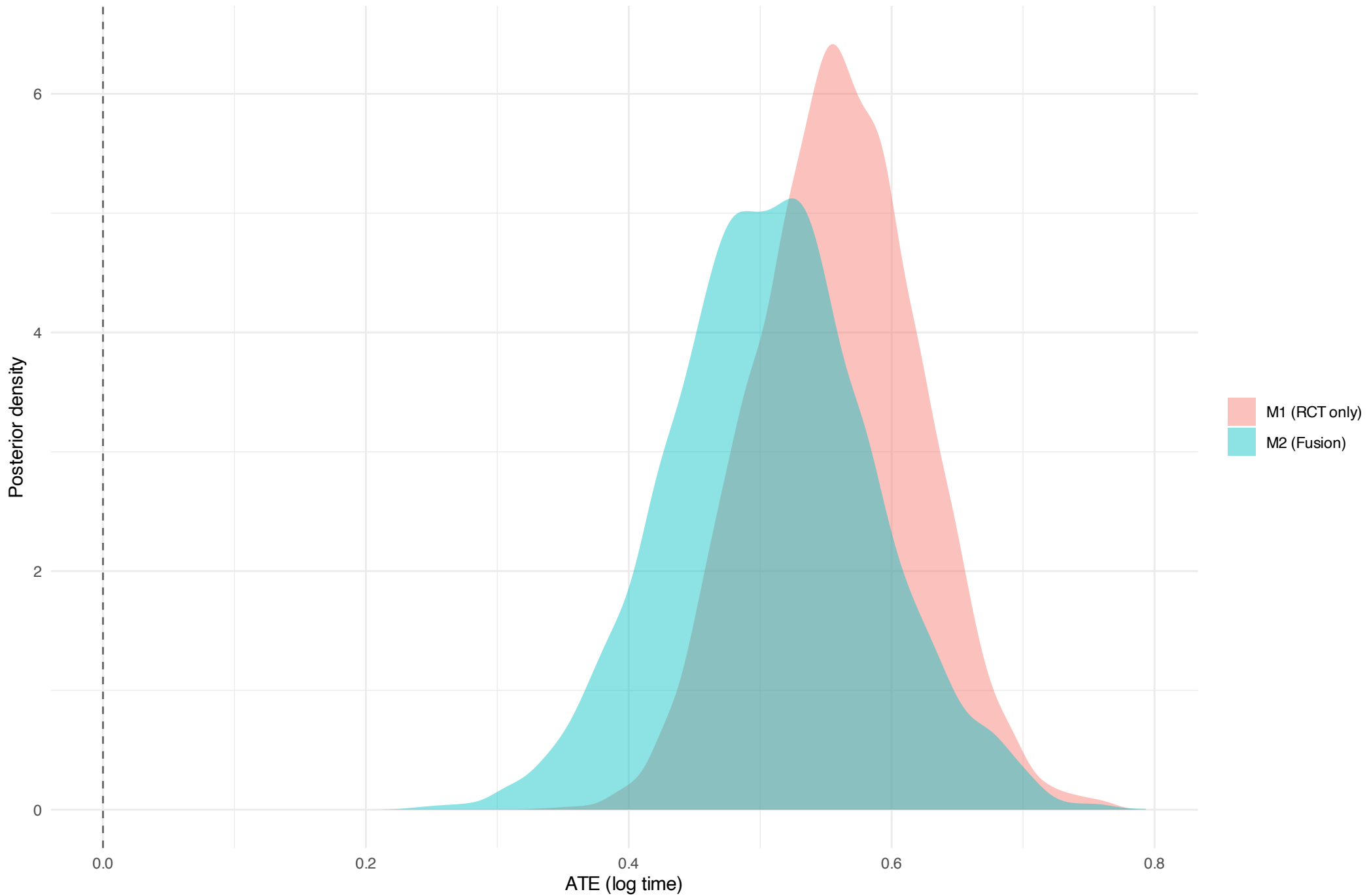
Average treatment effect on the RCT covariate distribution
