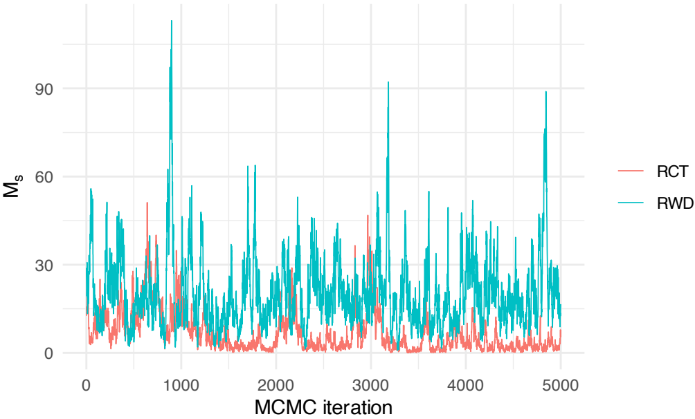
Occupied HDP components per source ( \pi_i > 0.01 )
